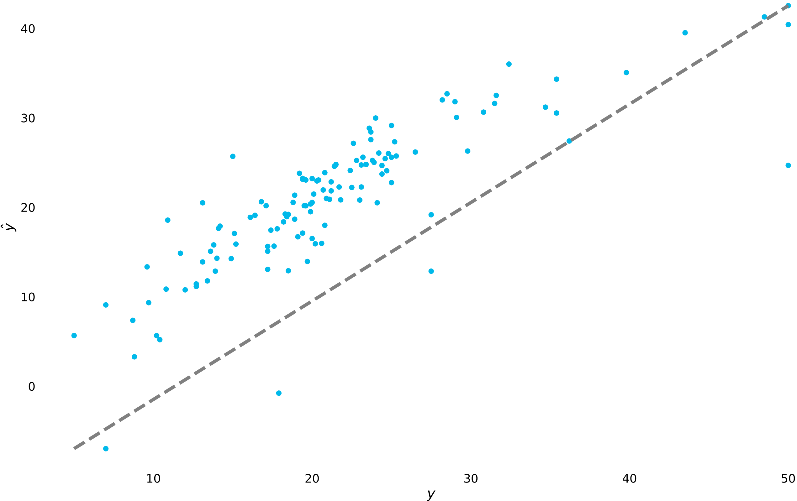
Prediction Error - LinearRegression
